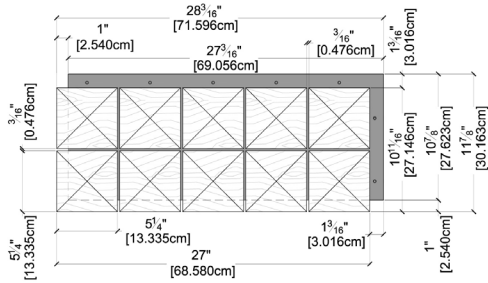
TOP VIEW DIMENSIONS
