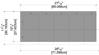
BOTTOM VIEW DIMENSIONS
