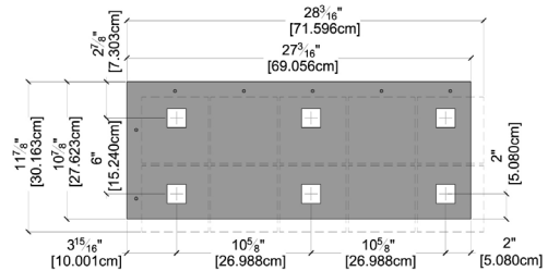
BOTTOM VIEW DIMENSIONS
